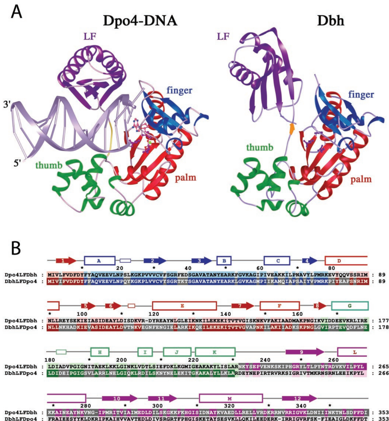
FIG. 1. Structures of the Dpo4 and Dbh proteins and generation of Dpo4/Dbh chimeras. A , ribbon diagram (34) of Dpo4 complexed with DNA and Dbh in the absence of DNA. The location of the four structural domains in Dpo4 (9) and Dbh (10, 21) are color coded as follows: red , palm domain; green , thumb domain; blue , finger domain; purple , little finger domain. A flexible linker tethers the LF and thumb domains of the polymerases. The orange arrow in Dbh represents a short \beta -strand that occurs in the middle of the linker region. This \beta -strand pins the LF domain to the palm domain by hydrogen bonds through the main chain atoms. The corresponding segment in Dpo4 is an extended loop that traverses the DNA backbone as shown in yellow . B , alignment of the Dpo4-LF-Dbh and Dbh-LF-Dpo4 chimeras. The finger, thumb, palm, and little finger domains are color coded as described above, and the secondary structures are indicated as boxes ( \alpha -helices) and arrows ( \beta -sheets) above the aligned primary amino acid sequence. Residues that are identical in Dpo4 and Dbh are highlighted. The primary amino acid sequence of Dpo4 is shown in a black typeface on a light gray background , whereas that of Dbh is shown in a white typeface on a dark gray background . Dpo4-LF-Dbh consists of Dpo4 finger, palm, and thumb residues and the LF domain from Dbh. Dbh-LF-Dpo4 consists of Dbh finger, palm, and thumb residues and the LF domain of Dpo4. Asterisk or number indicates every other tenth residue.
